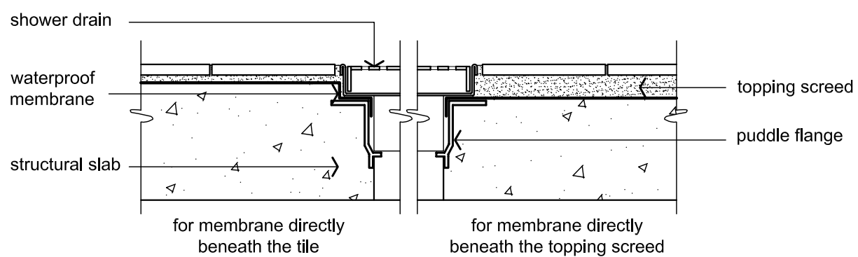
INSTALLATION DETAIL
